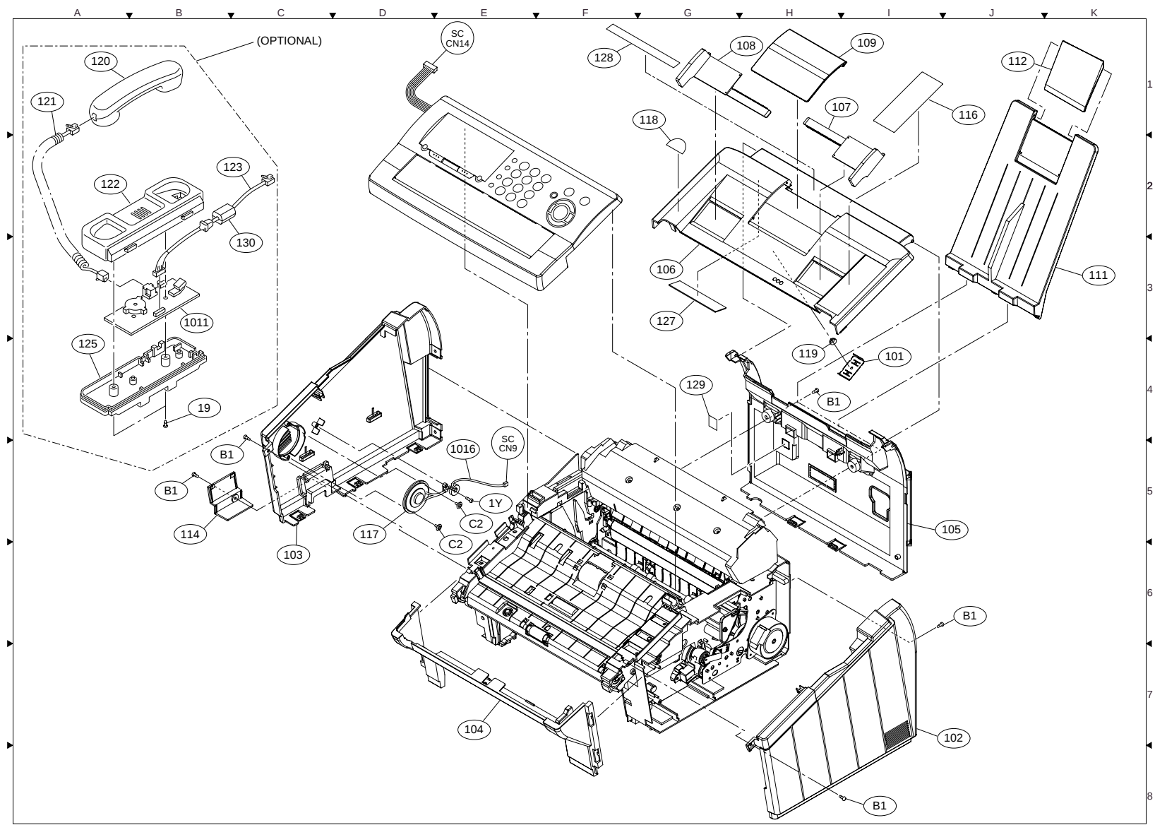
FIG. 1 COVER ASSEMBLY
