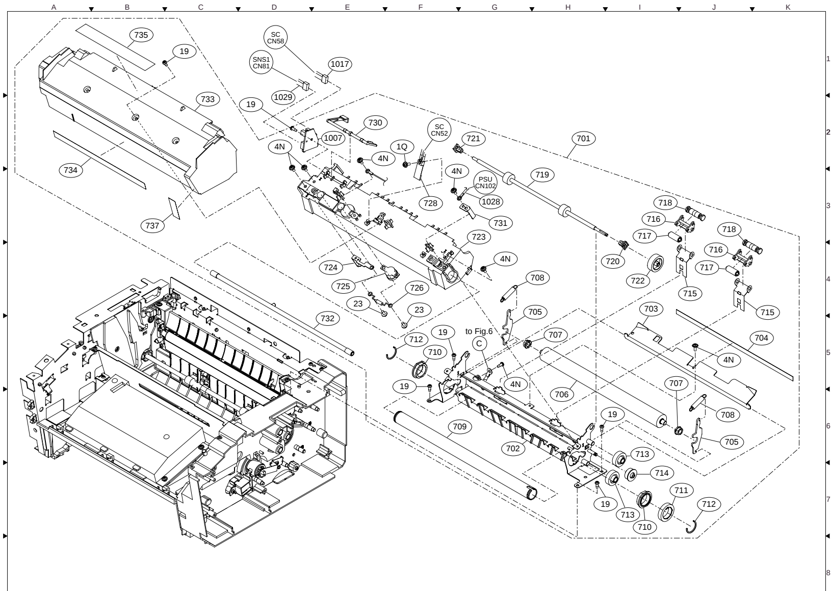
FIG. 7 FUSER UNIT
