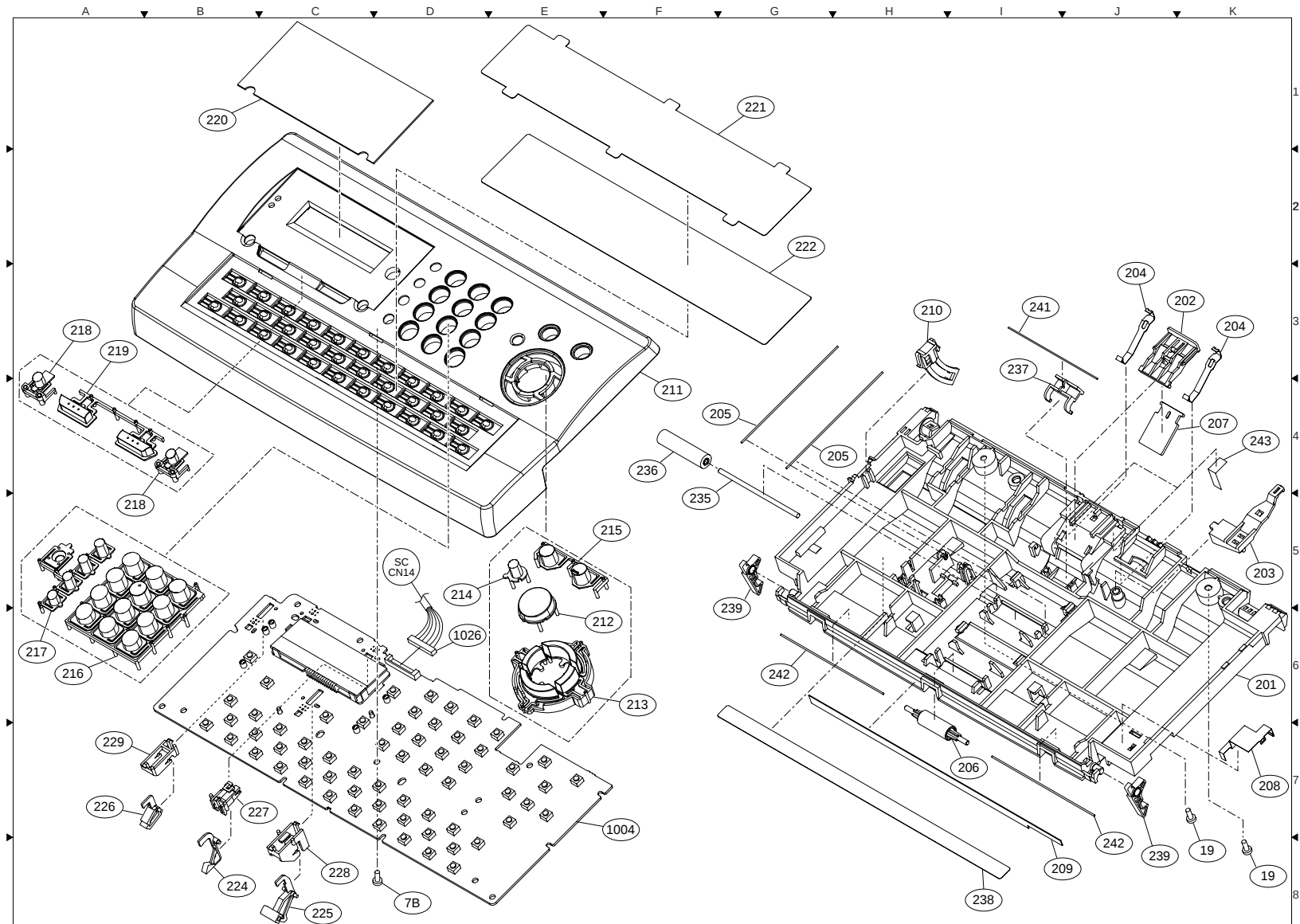
FIG. 2 CONTROL PANEL UNIT
