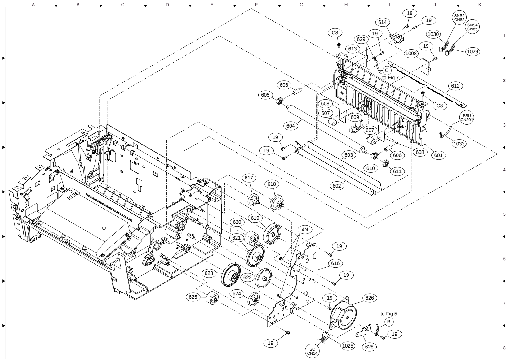
FIG. 6 PAPER TRANSPORTATION
