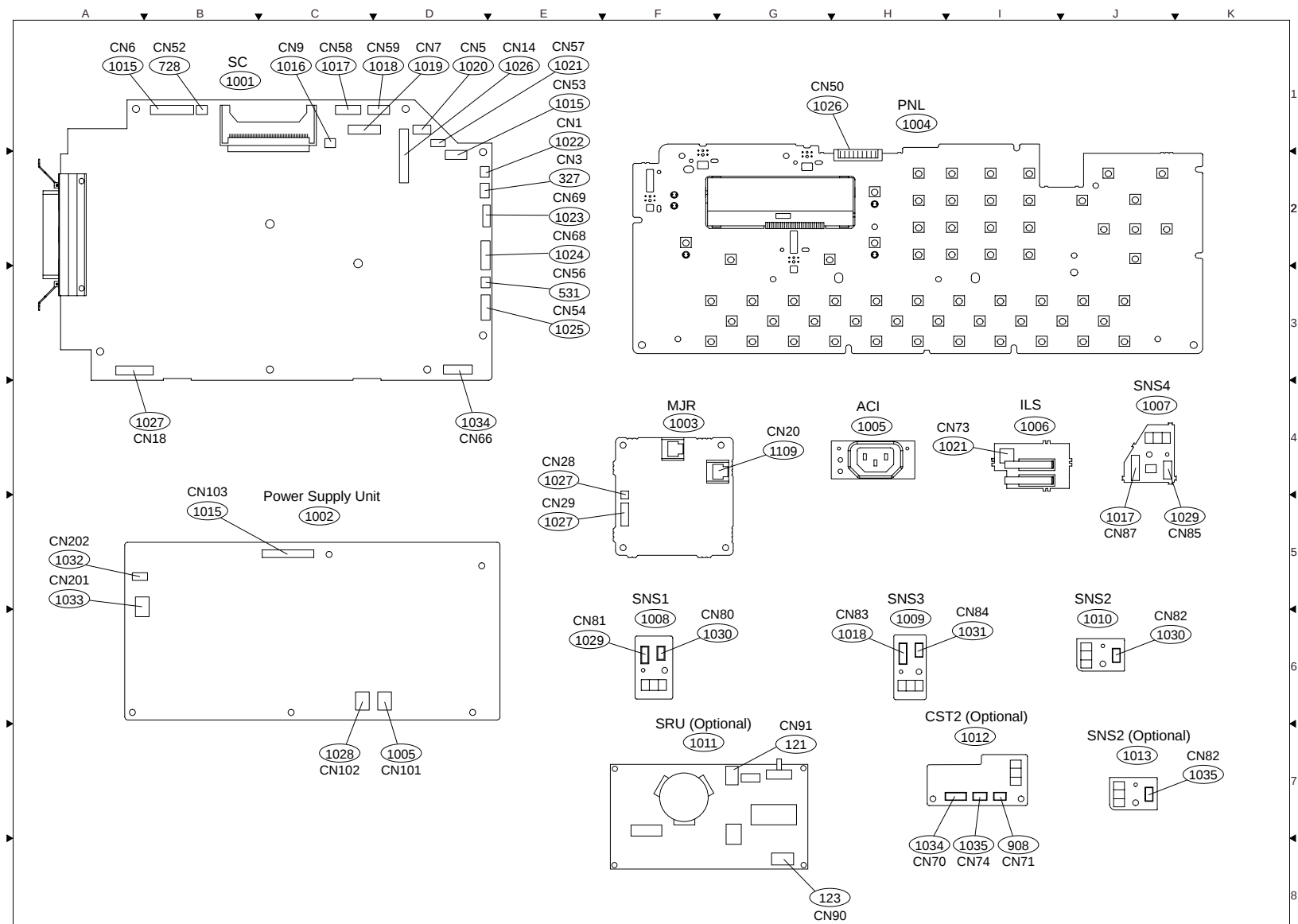
FIG. 10 PC BOARD / HARNESS
