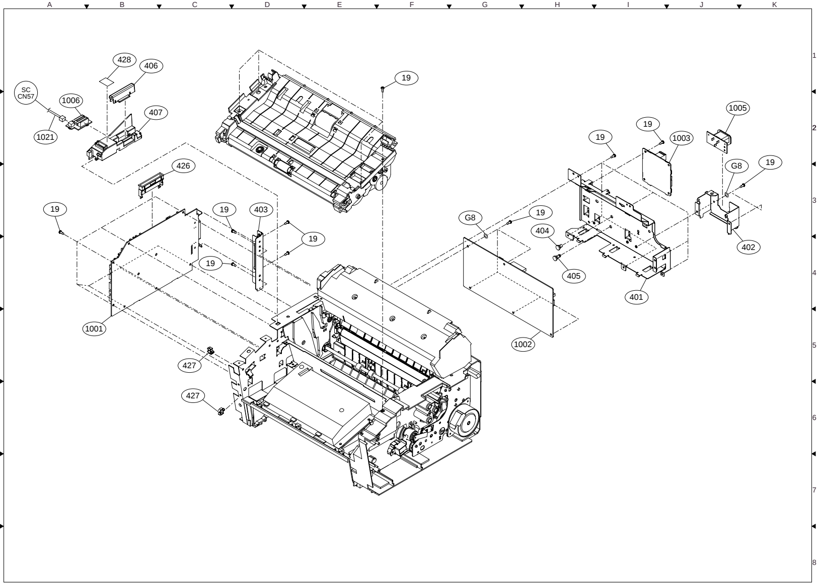
FIG. 4 ELECTRICAL PARTS
