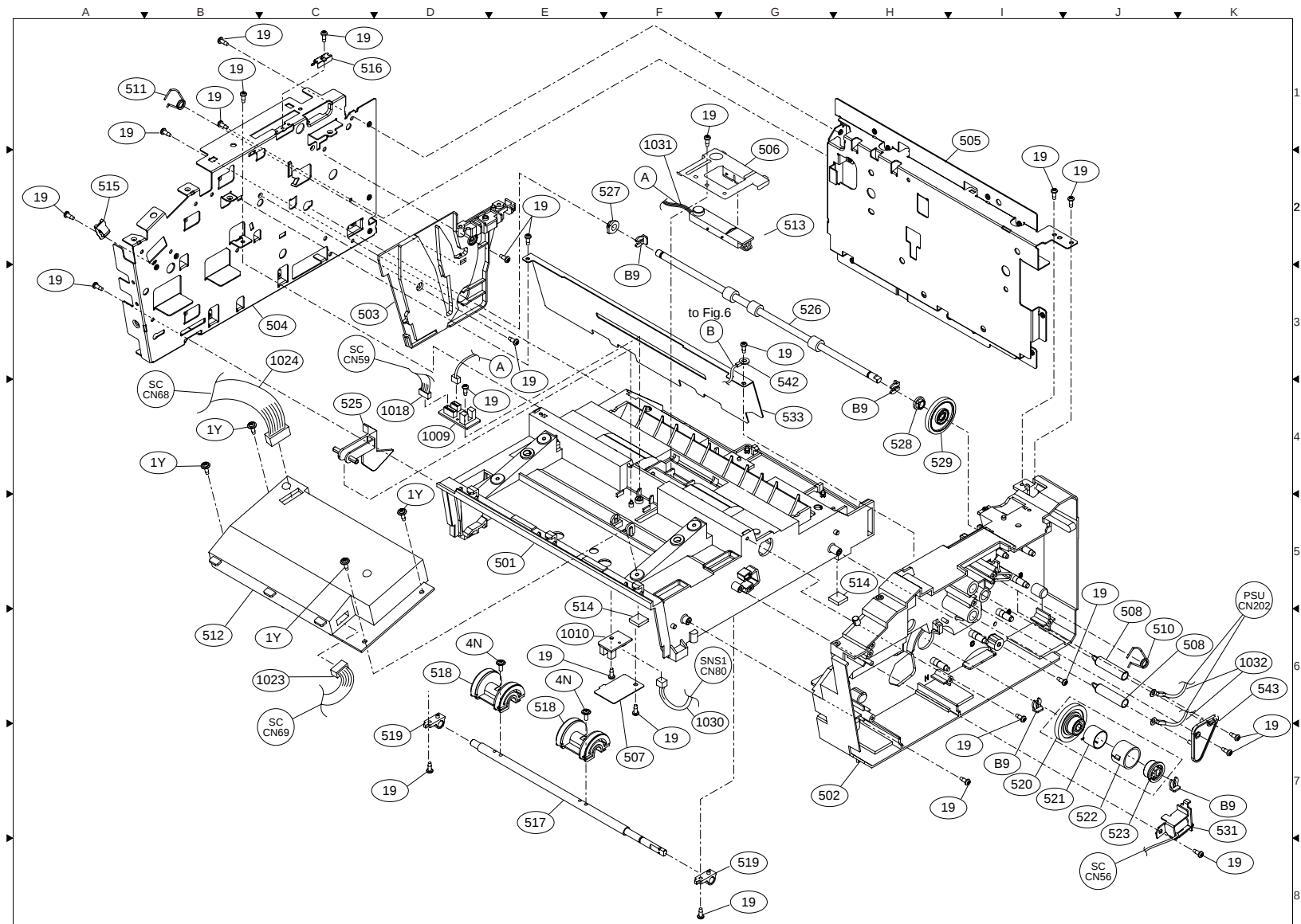
FIG. 5 BASE UNIT
